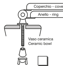
Cerniere per vaso con fori passanti Hinges for toilet with through holes
